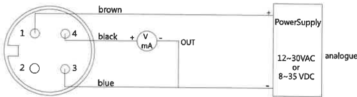
4P M12 Connector + Analogue
